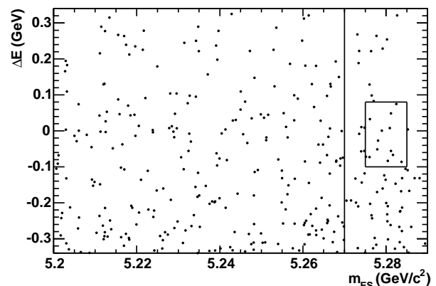
FIG. 2: Distribution of data events in the \Delta E - m_{ES} plane. The lines indicate the regions of the signal box and of the grand sideband.
