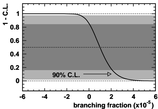
FIG. 4: 1–confidence level versus the assumed branching fraction. The shaded areas are the 68% and 95% probability regions. The 90% C.L. is marked with an arrow.
