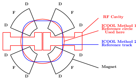
Fig. 1. A way of fitting a pair of large 201 MHz RF cavities into a small four sector cyclotron. The cavities fill the center of the cyclotron.
